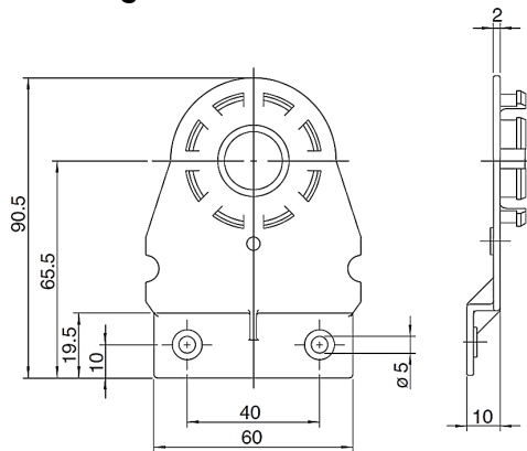
Mounting bracket 6482
